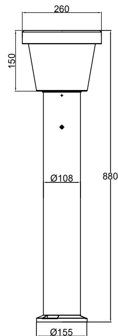
LED
